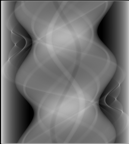
Original Sinogram
