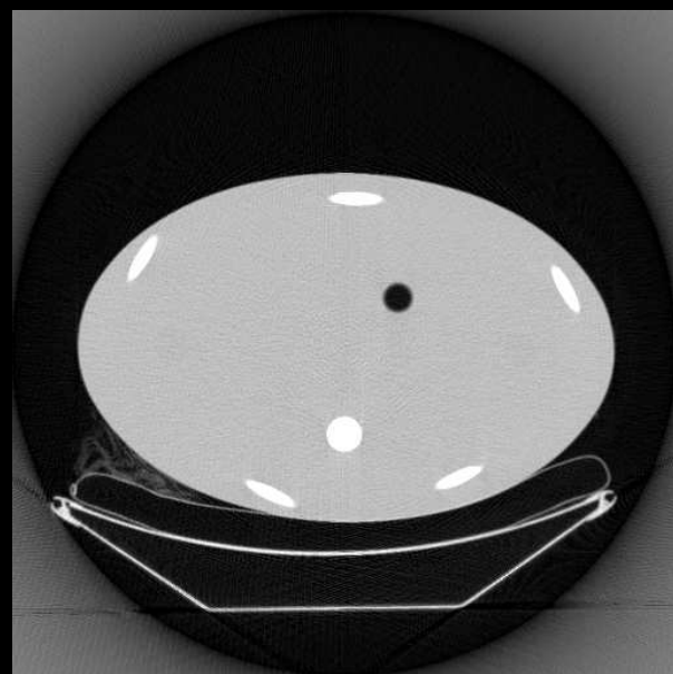
CT Phantom
