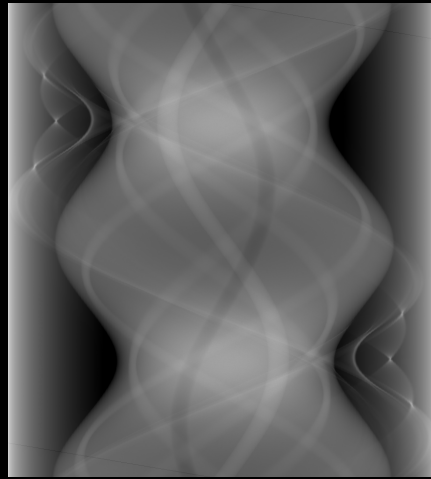
Rebinned Sinogram
